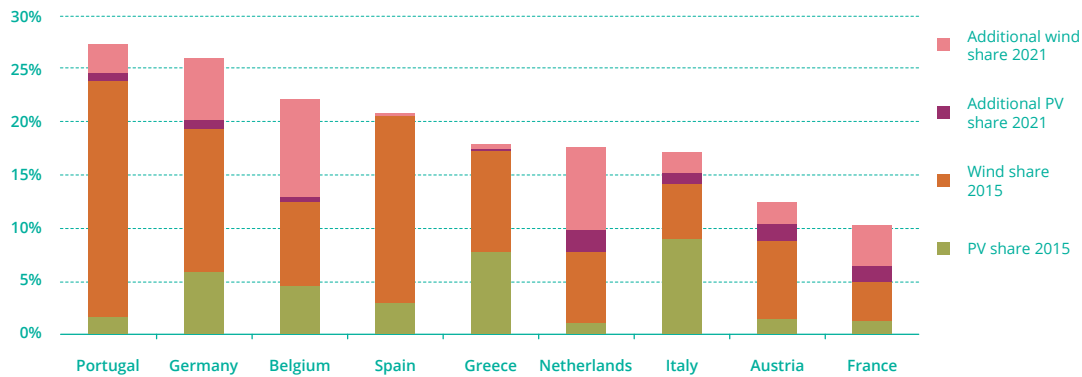
Share of VRE generation in 2015 and 2021 for selected UCTE countries
