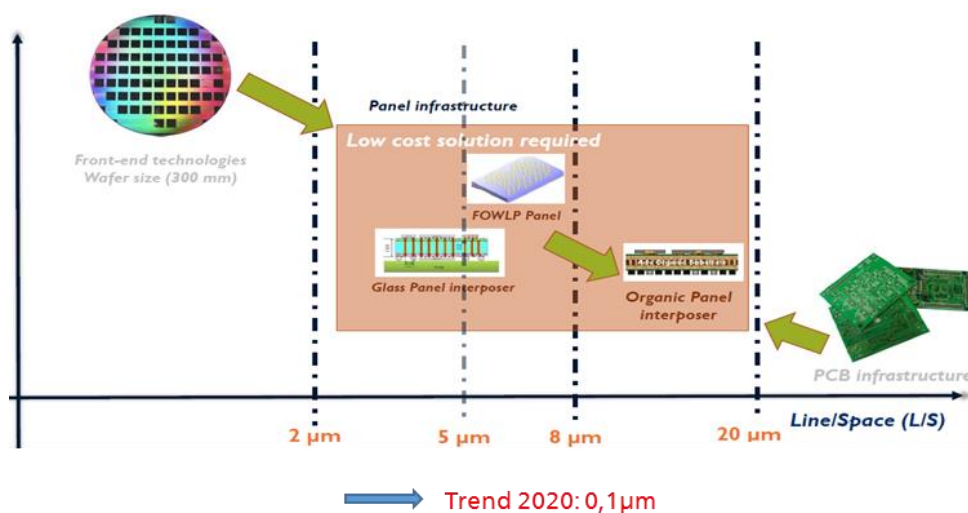
Figure 4 - The heterogeneous integration domain in electronic components merges the conventional PCB with the wafer level technologies (source: Fraunhofer IZM).
