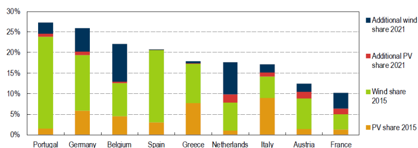
Figure 27 - Share of VRE generation in 2015 and 2021 for selected UCTE countries
