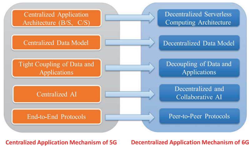
FIGURE 2. Evolution of 6G decentralized application provisioning.
